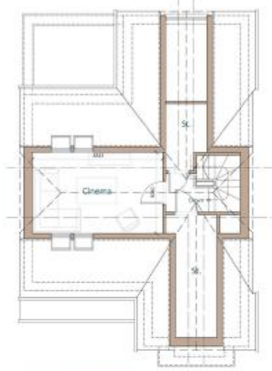
Proposed Second Floor Plan Scale 1:50
